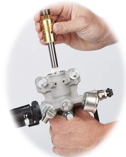
4. Replace cartridge
