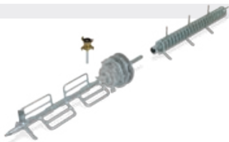
Fine mortar mixing kit (standard for Spin 15A Cappotto version)
